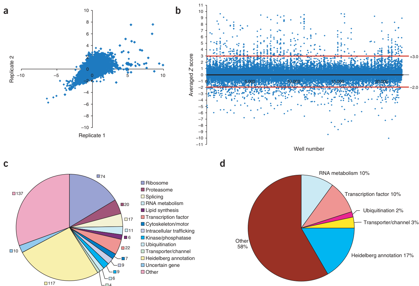
Figure 2 Primary screen results. (a) Correlation of replicate Z scores for the first five primary screening plates. The data in a and b were filtered to remove values greater than +10.0, which correspond to the artificially high normalized values found in some edge wells. (b) Scatter plot of all averaged Z scores from the primary screen. Red lines indicate -2.0 and +3.0 averaged Z score thresholds. Each screening plate contained four control wells, one of which contained smo dsRNA. These smo control wells formed the majority of the data points with Z scores near -5.0 . (c) Functional classification of the 449 genes with Z scores less than -2.0 when reduced by RNAi in the Hh signaling assay. These genes are likely to function as positive regulators of Hh signaling. Numbers of genes in each category are indicated. (d) Functional classification of the 60 genes with Z scores greater than +3.0 when reduced by RNAi in the Hh signaling assay. These genes are likely to function as negative regulators of Hh signaling.
